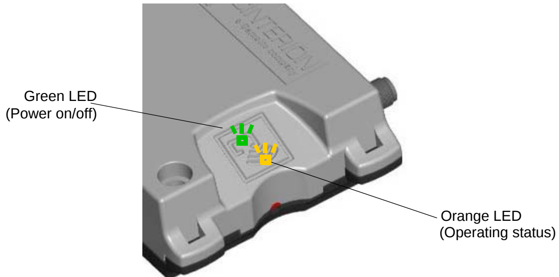
Figure 9: Status LED
